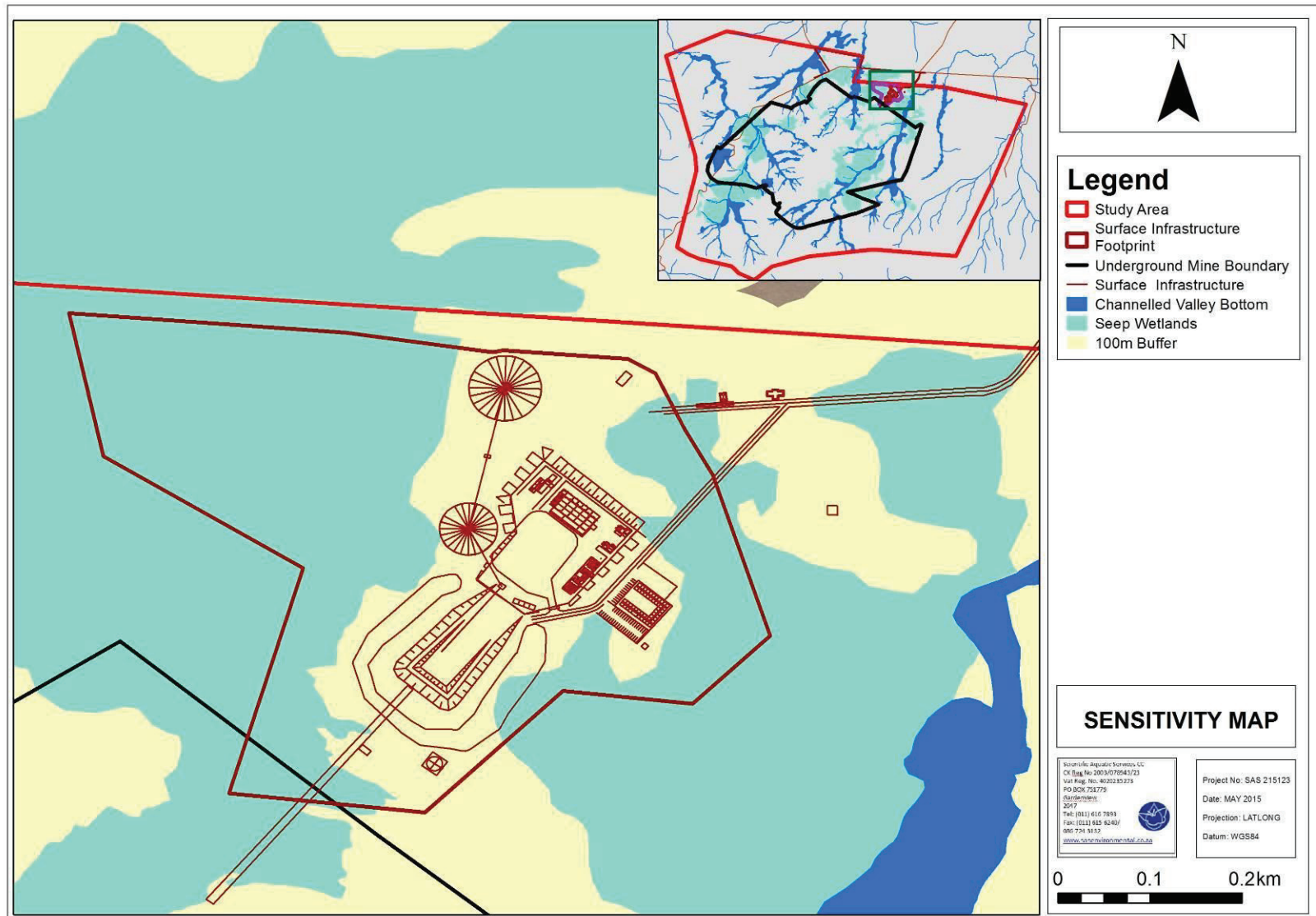
Figure 38: Conceptual representation of the wetland systems assessed within the surface infrastructure footprint with the associated 100m buffer zone.
