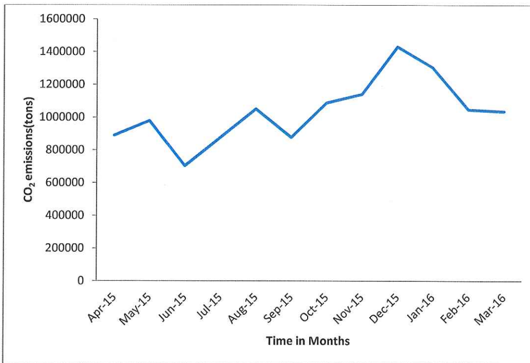
Figure 4. Monthly CO 2 Emissions in tons from Arnot Power Station 2015/2016
