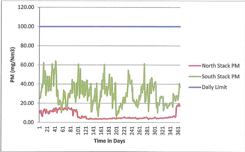
Figure 1. Daily Particulate Emissions in mg/Nm 3 from Arnot Power Station for 2015/2016
