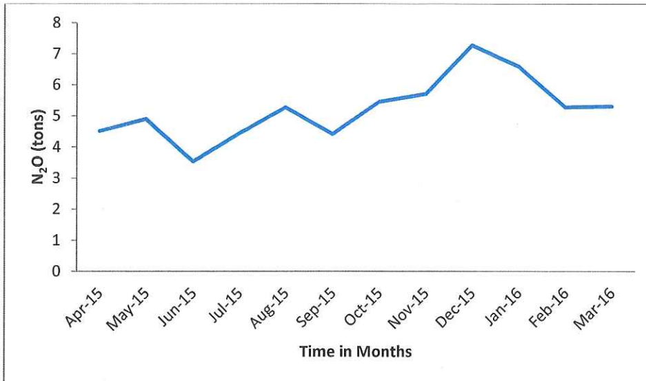
Figure 5. Monthly N 2 O Emissions in tons from Arnot Power Station 2015/2016
