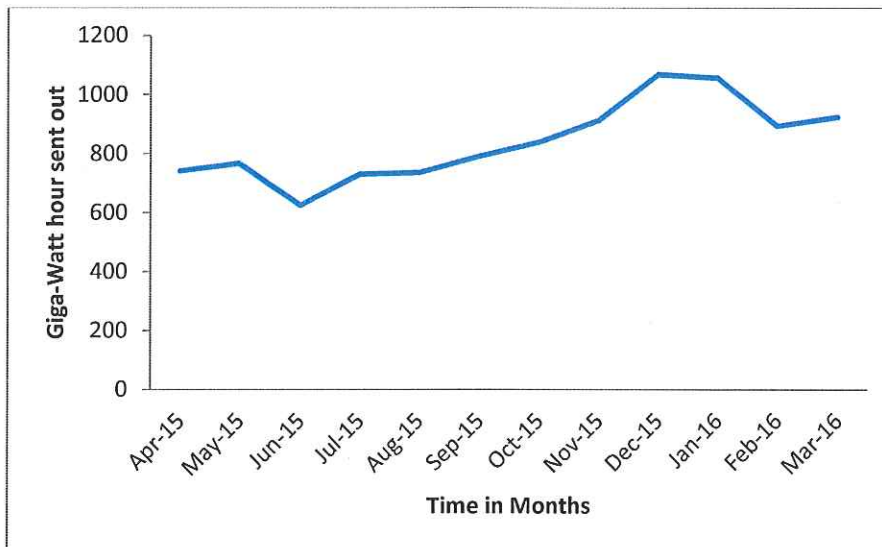
Figure 6. Monthly Energy sent out in GWh at Arnot Power Station 2015/2016
