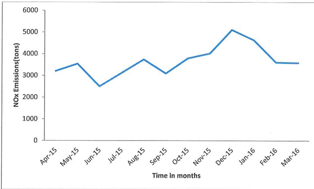
Figure 3. Monthly NO 2 Emissions in tons for Arnot Power Station 2015/2016
